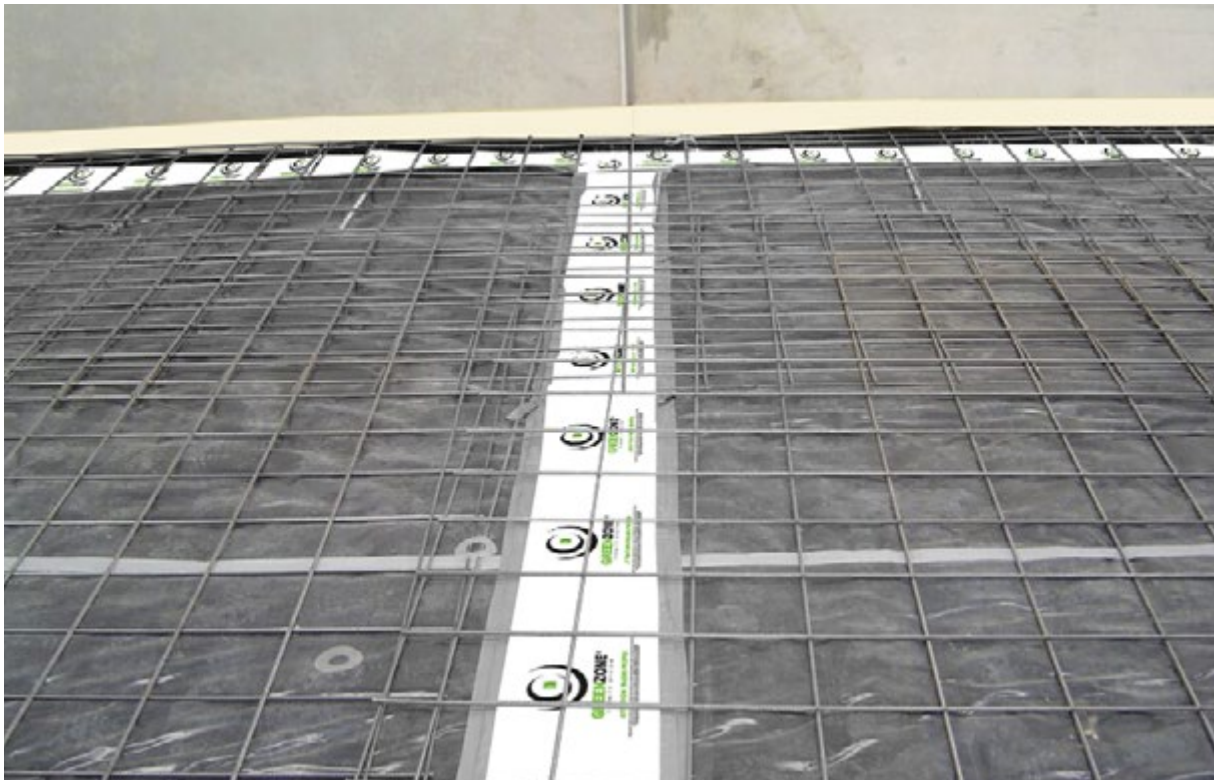
FIGURE 9.7 B GREENZONE® Perimeter Termite System (PTS) (300mm wide) is installed – taped horizontally to the moisture membrane. This is a concrete tilt up – the product is to overlap the internal perimeter protection. The detail for brick – veneer the product is installed onto the external brick work to overlap the GREENZONE® PTS installation.
